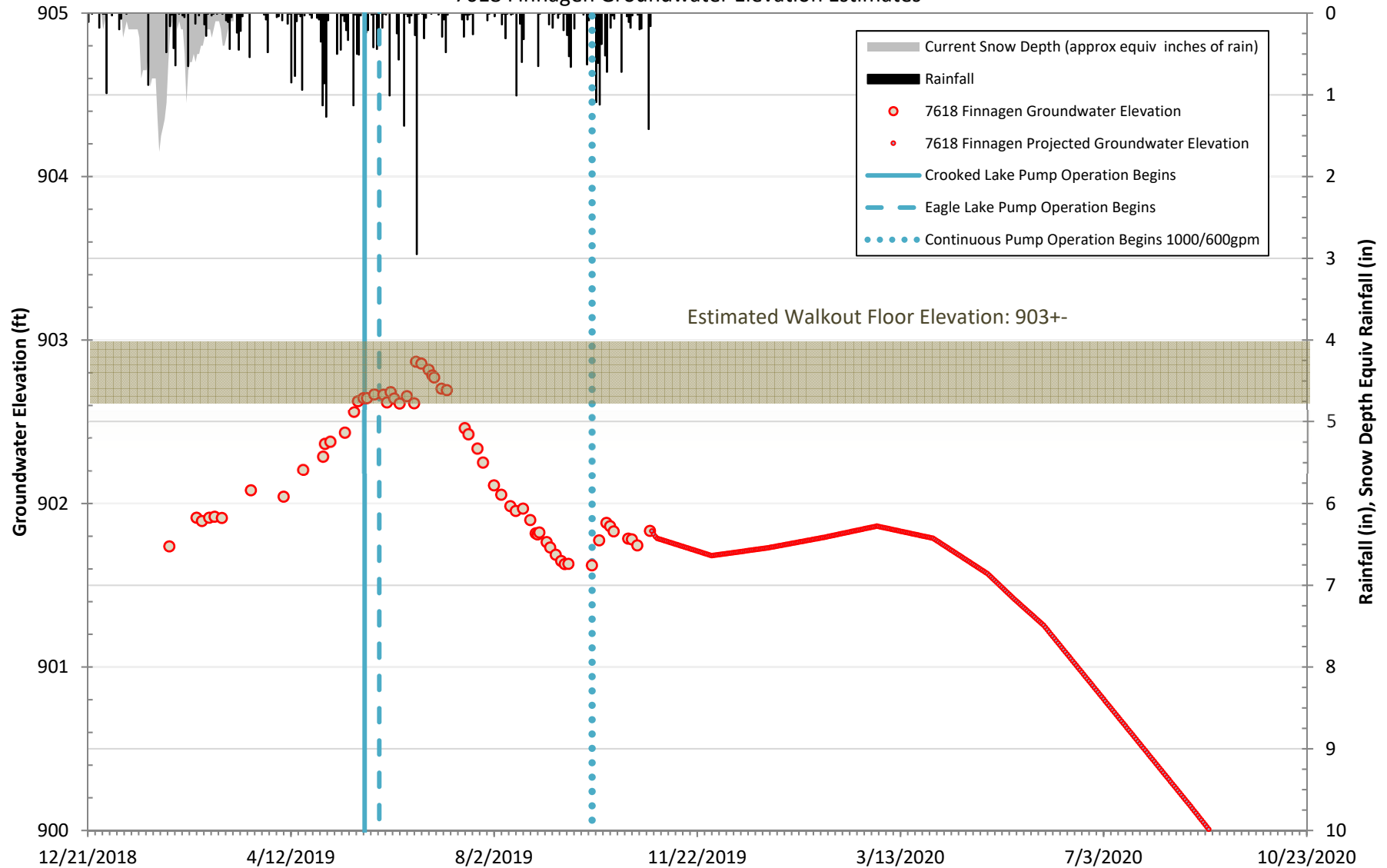
Charter Township of Texas Flood Study Figure 7618 Finnagen Groundwater Elevation Estimates
