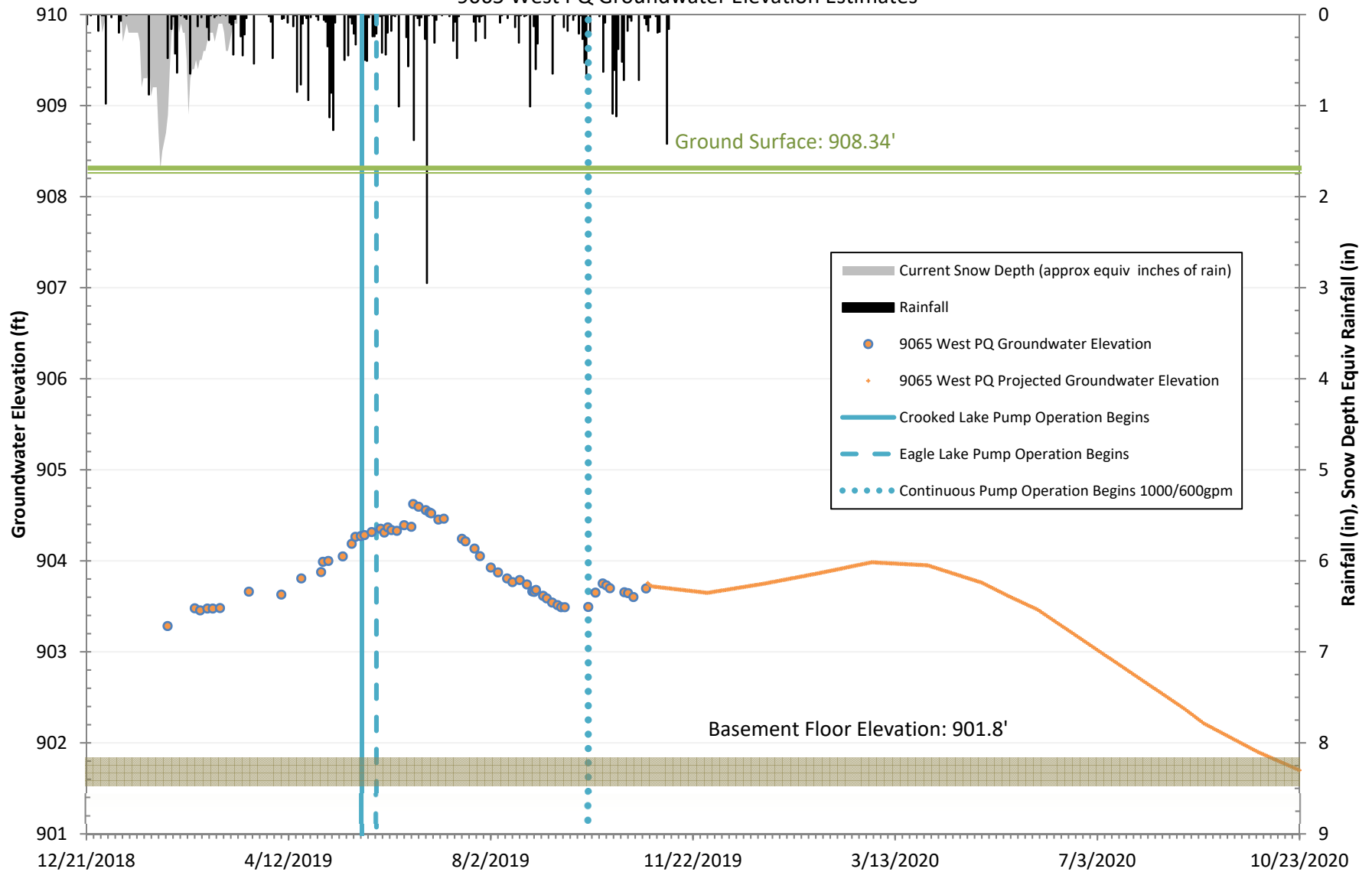
Charter Township of Texas Flood Study Figure 9065 West PQ Groundwater Elevation Estimates
