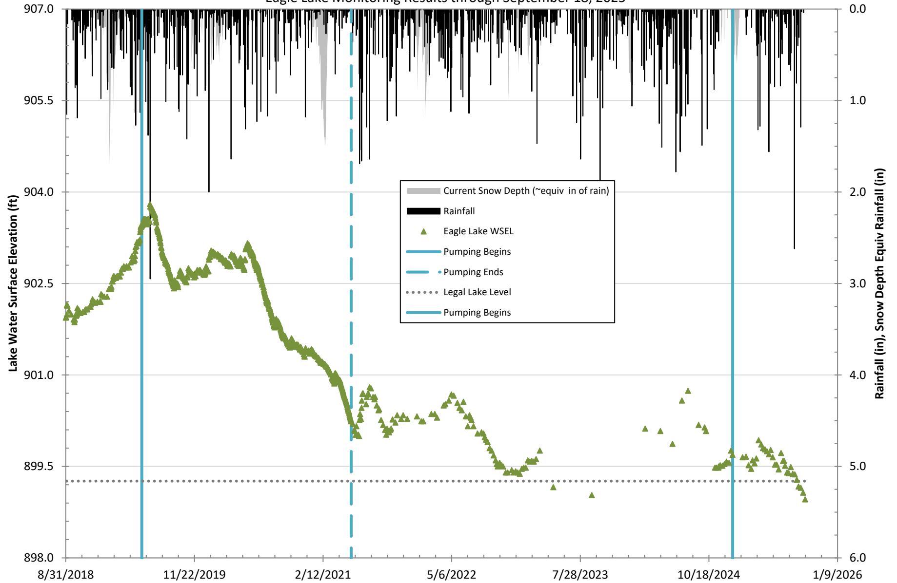
Charter Township of Texas Flood Study Figure Eagle Lake Monitoring Results through September 18, 2025
