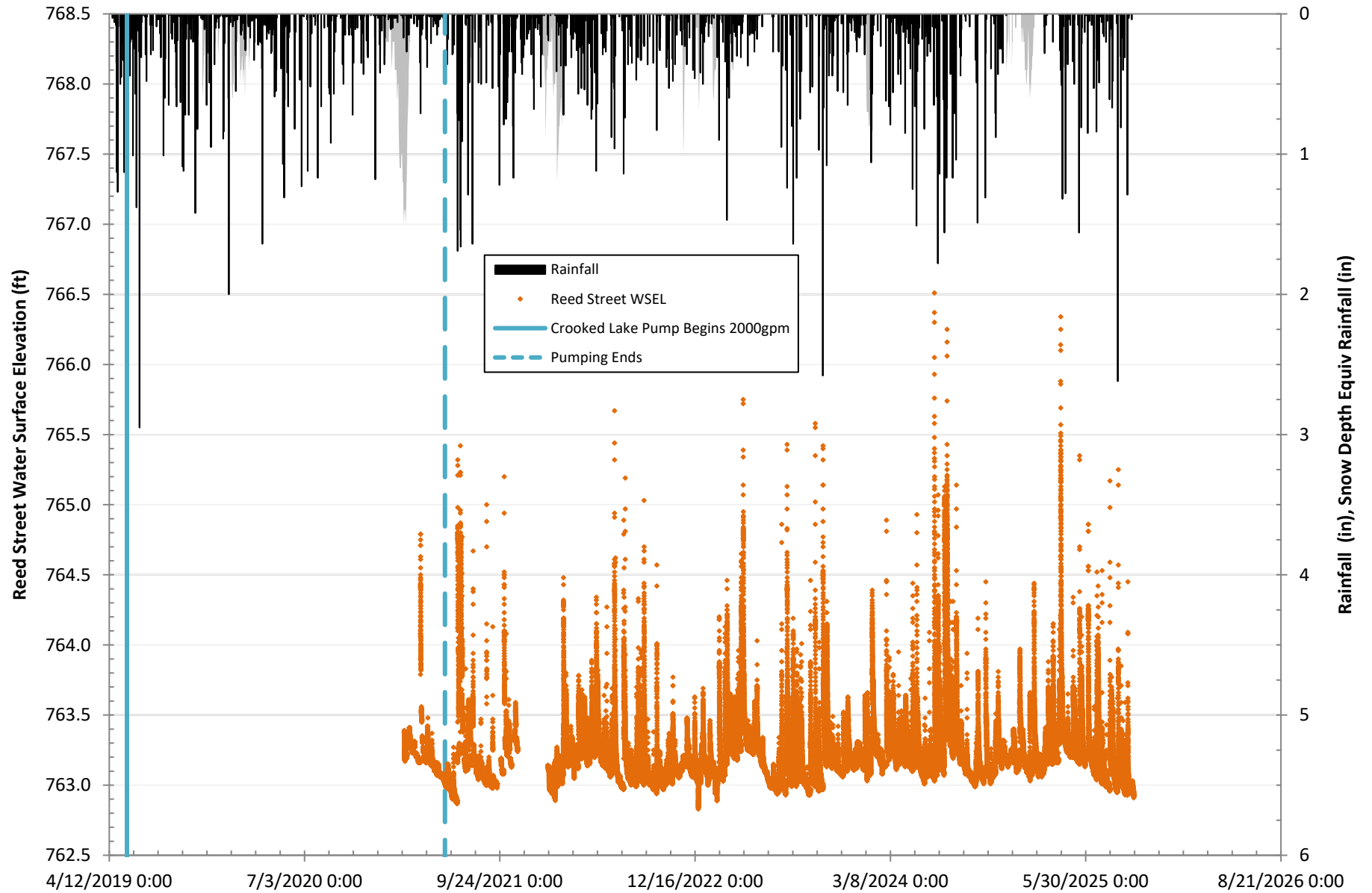
Charter Township of Texas Flood Study Figure Reed Street Monitoring Results through September 18, 2025
