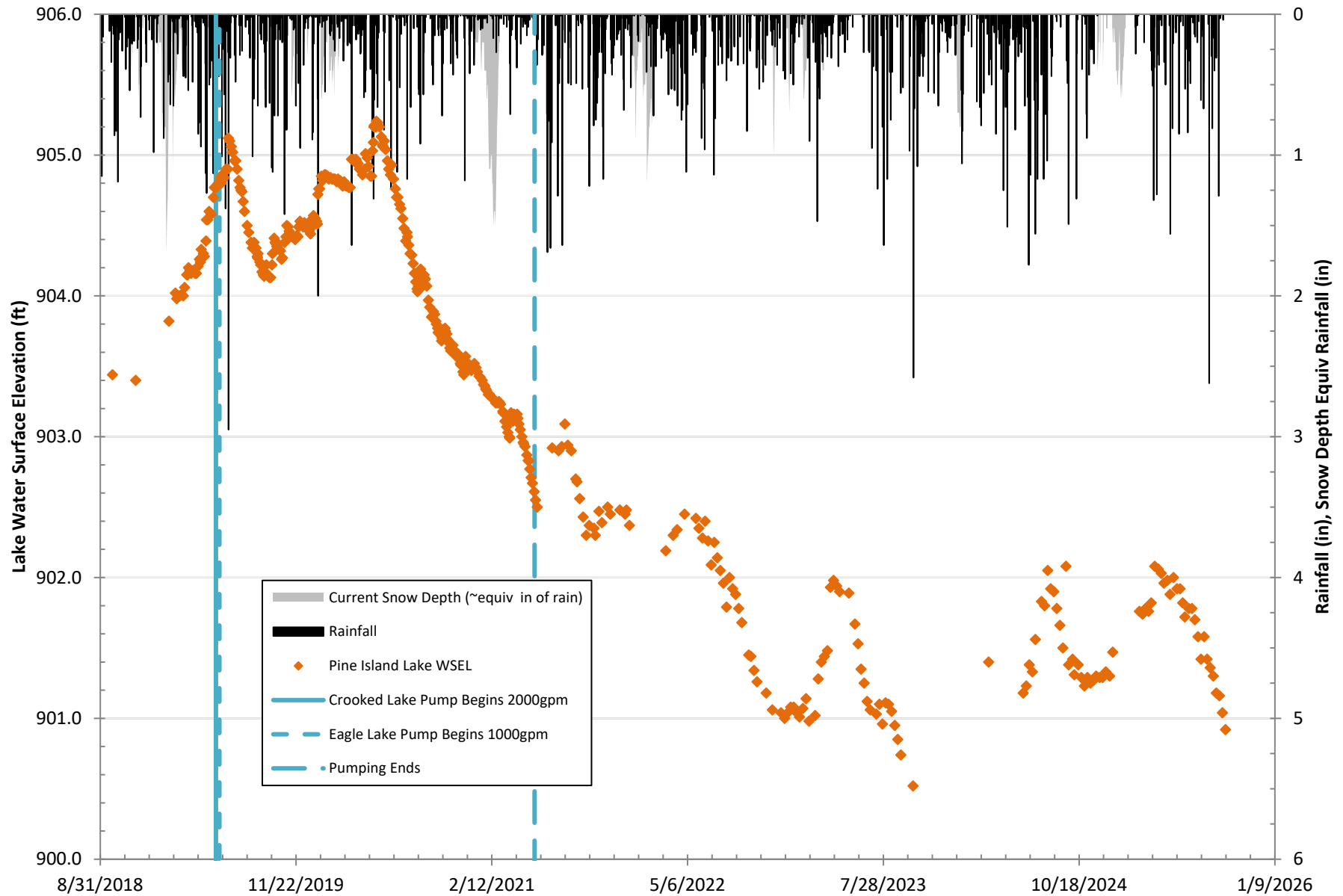
Charter Township of Texas Flood Study Figure Pine Island Lake Monitoring Results through September 18, 2025
