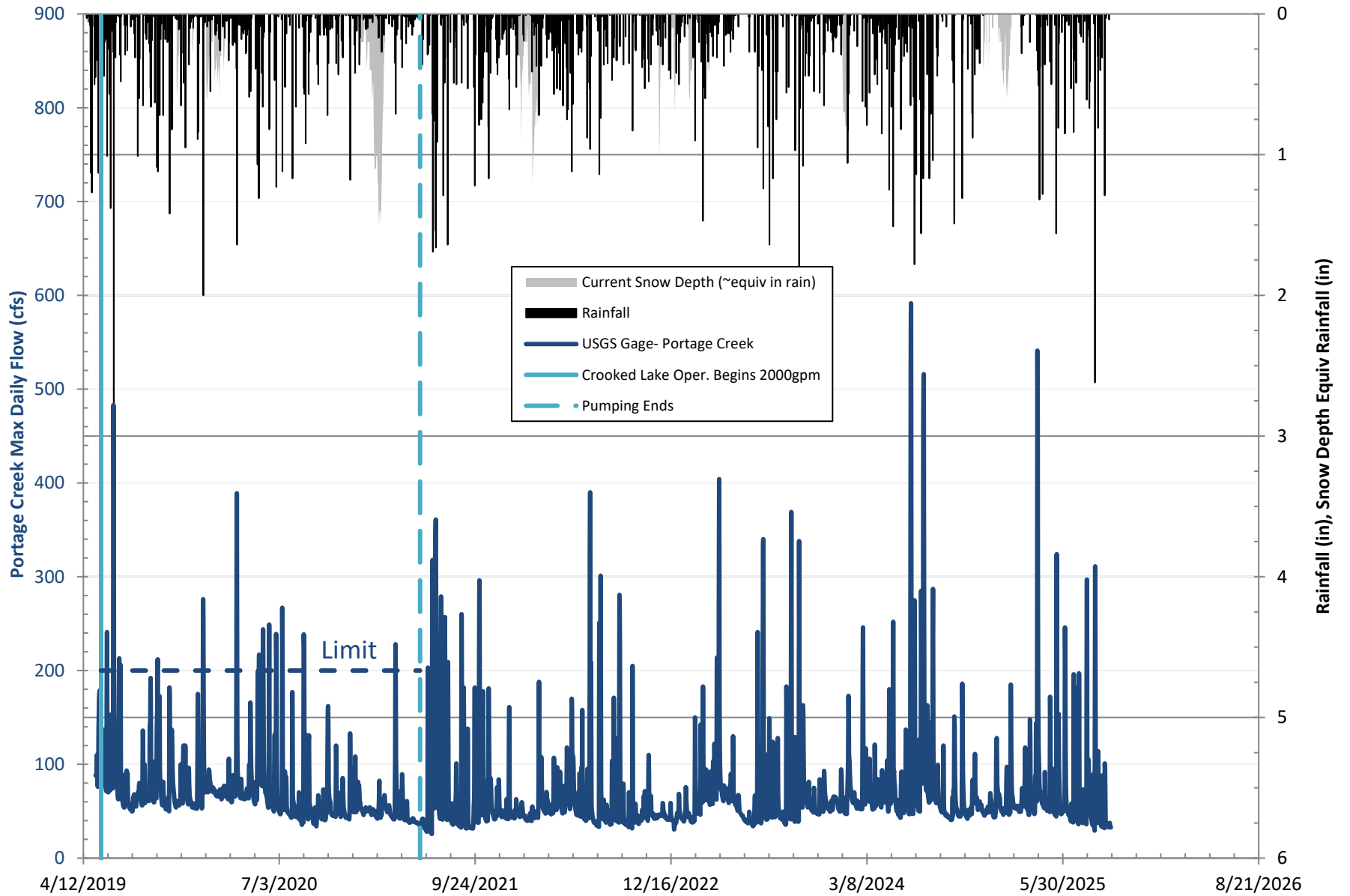
Charter Township of Texas Flood Study Figure USGS Portage Creek Monitoring Results through September 18, 2025
