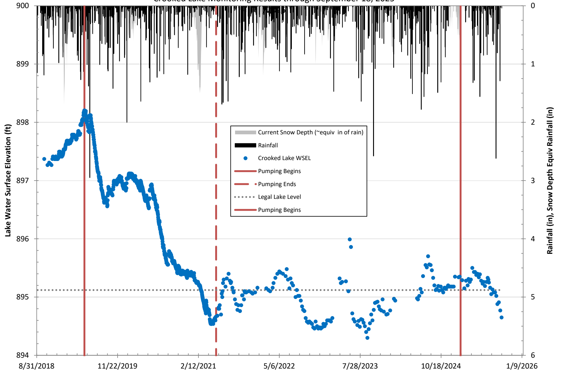
Charter Township of Texas Flood Study Figure Crooked Lake Monitoring Results through September 18, 2025
