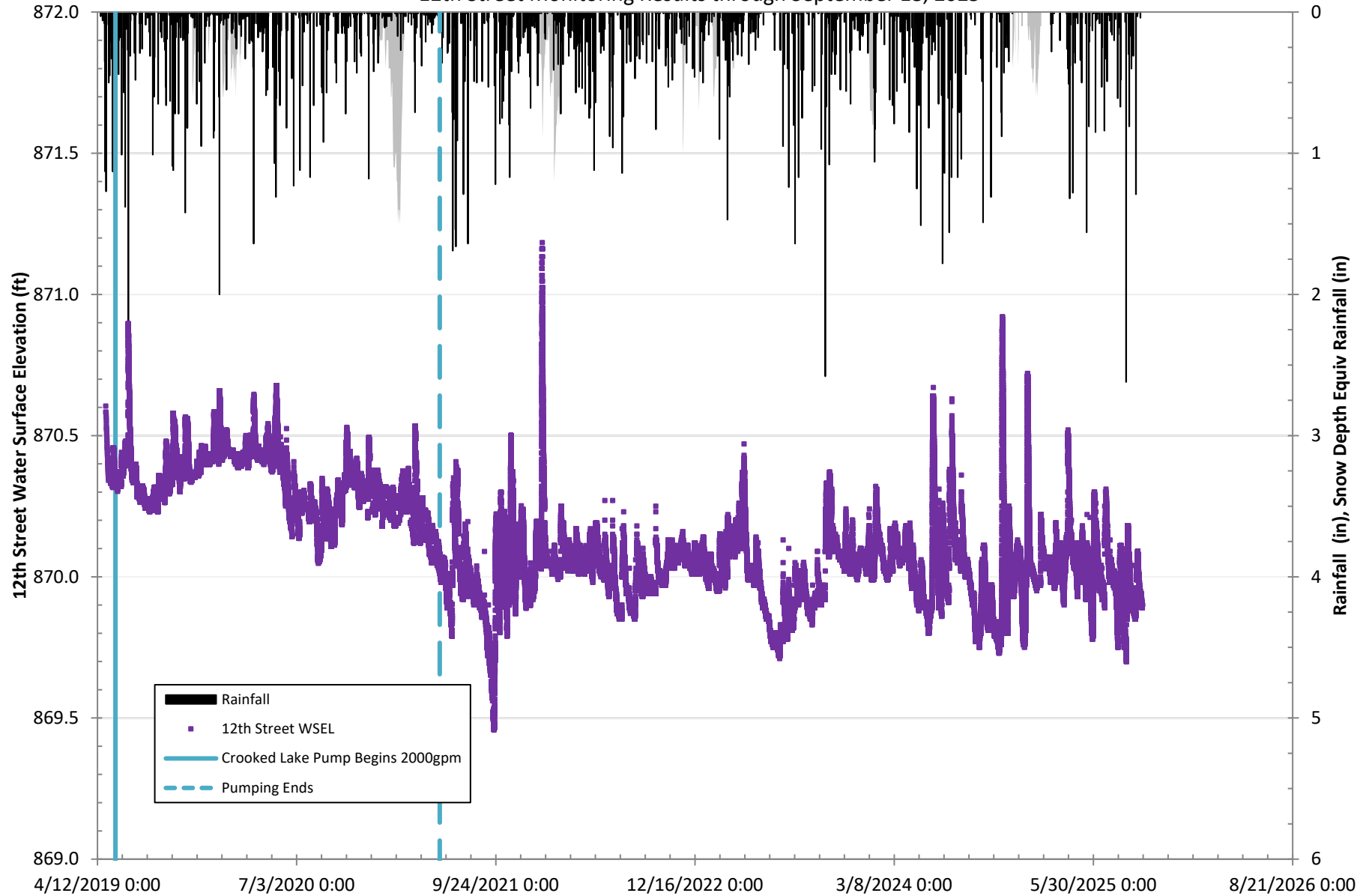
12th Street Monitoring Results through September 18, 2025
