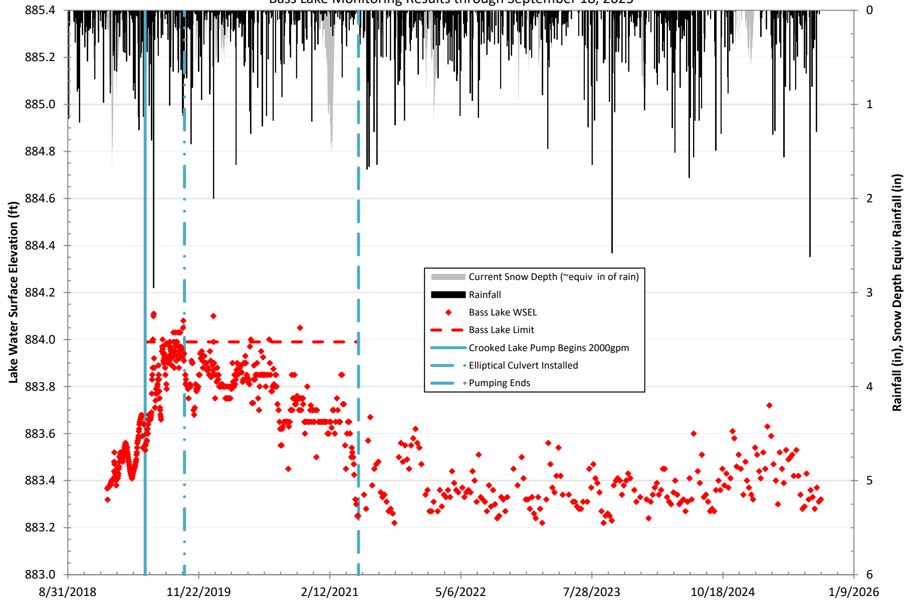
Charter Township of Texas Flood Study Figure Bass Lake Monitoring Results through September 18, 2025
