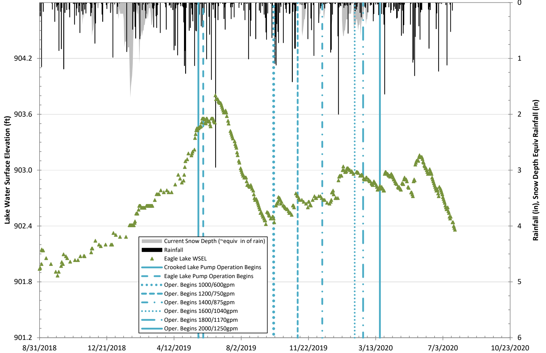
Charter Township of Texas Flood Study Figure Eagle Lake Monitoring Results through July 23, 2020
