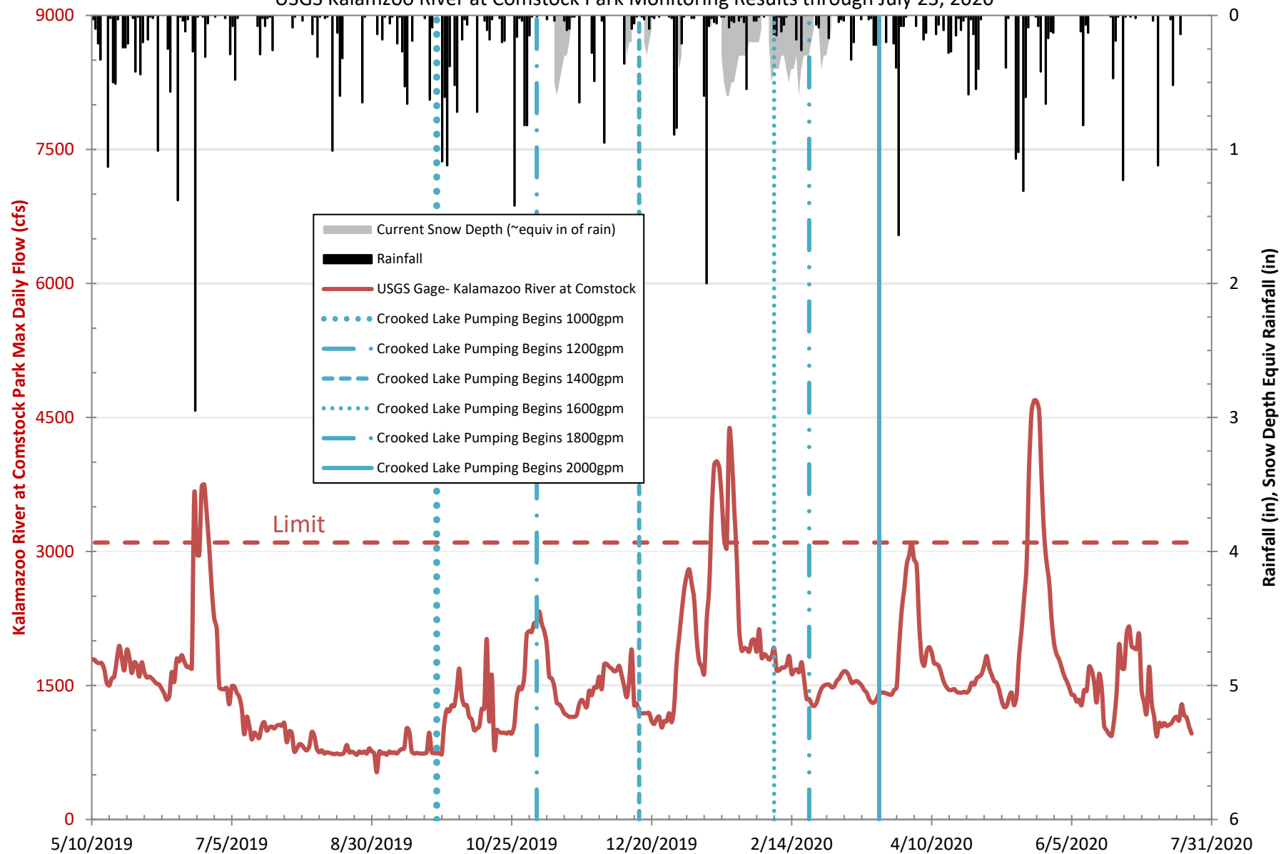
USGS Kalamazoo River at Comstock Park Monitoring Results through July 23, 2020
