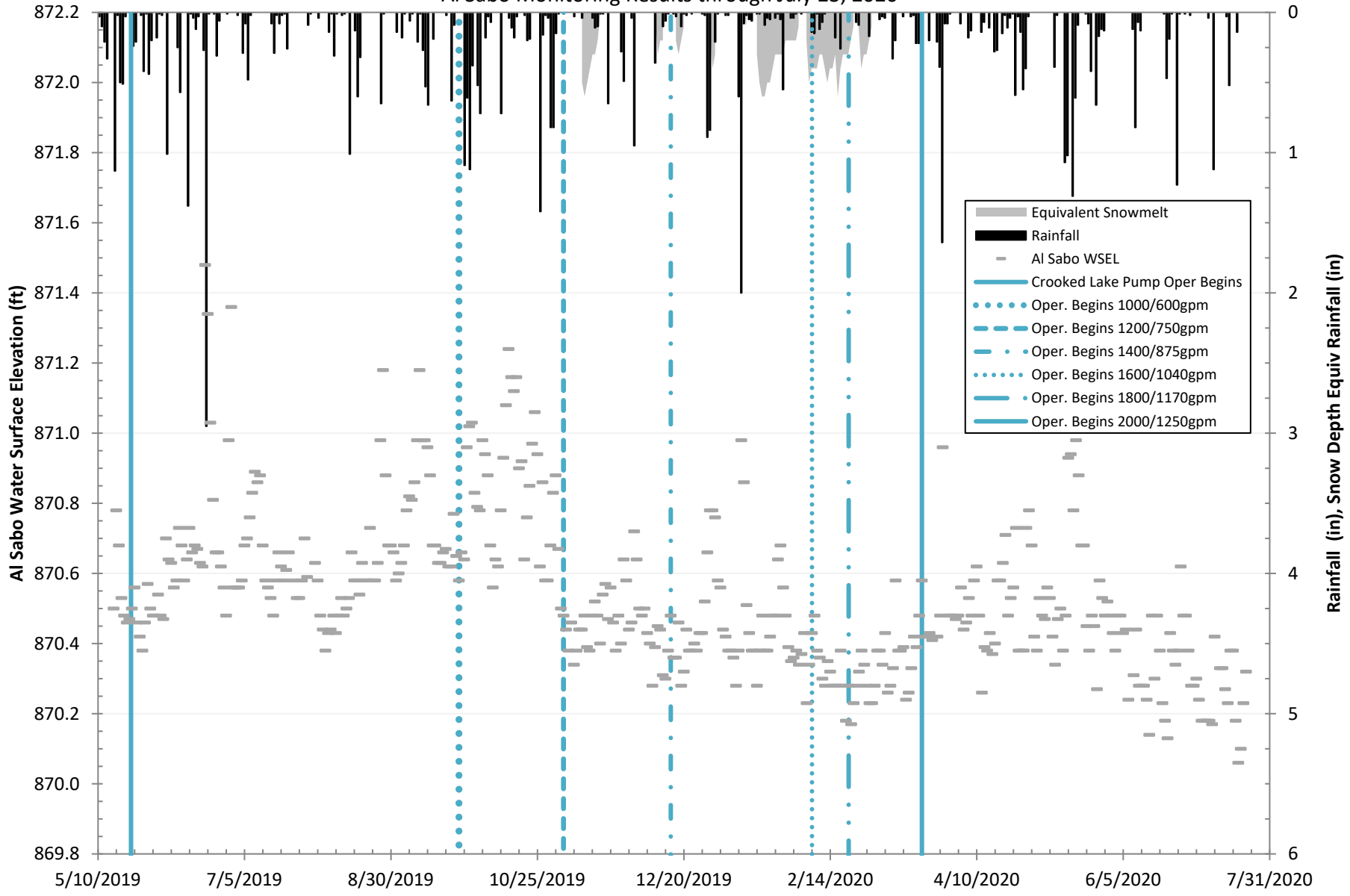
Charter Township of Texas Flood Study Figure Al Sabo Monitoring Results through July 23, 2020
