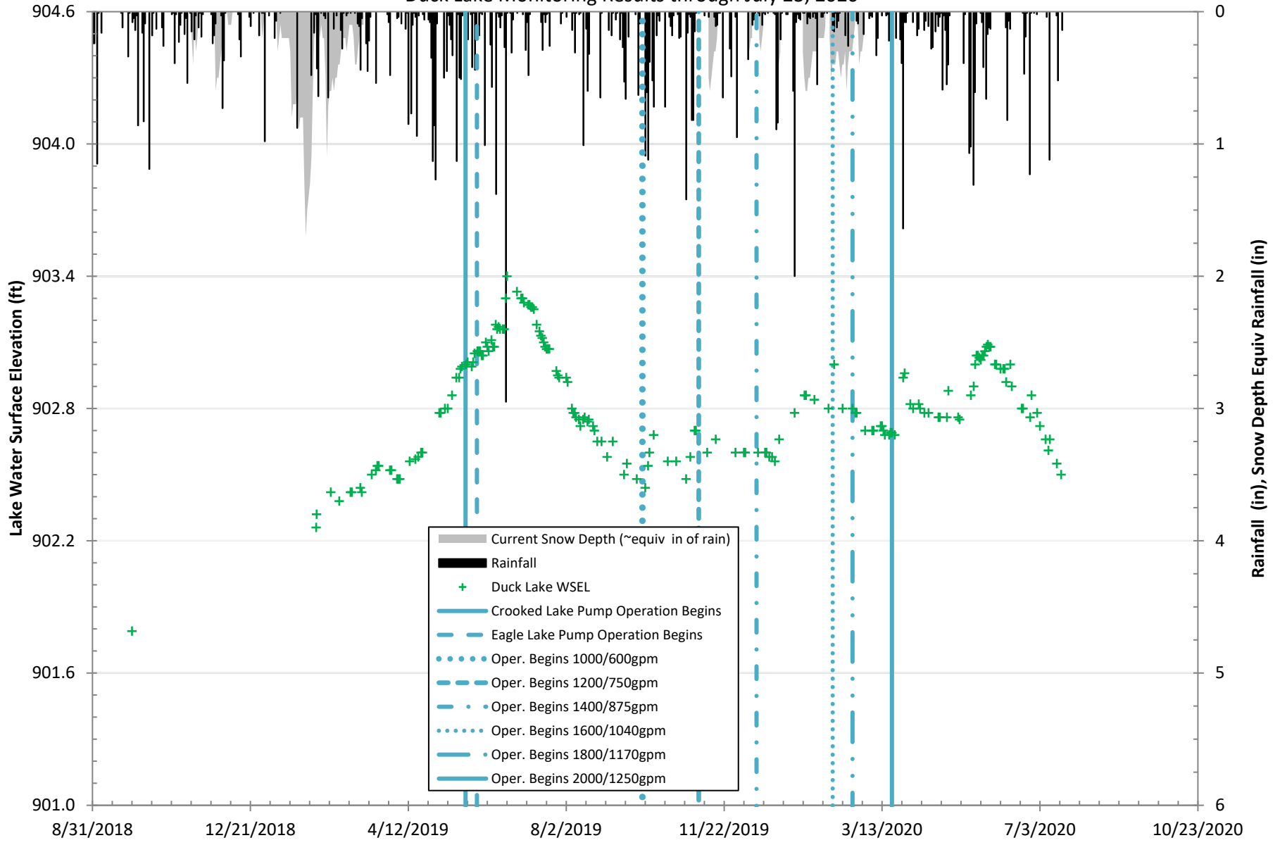
Charter Township of Texas Flood Study Figure Duck Lake Monitoring Results through July 23, 2020
