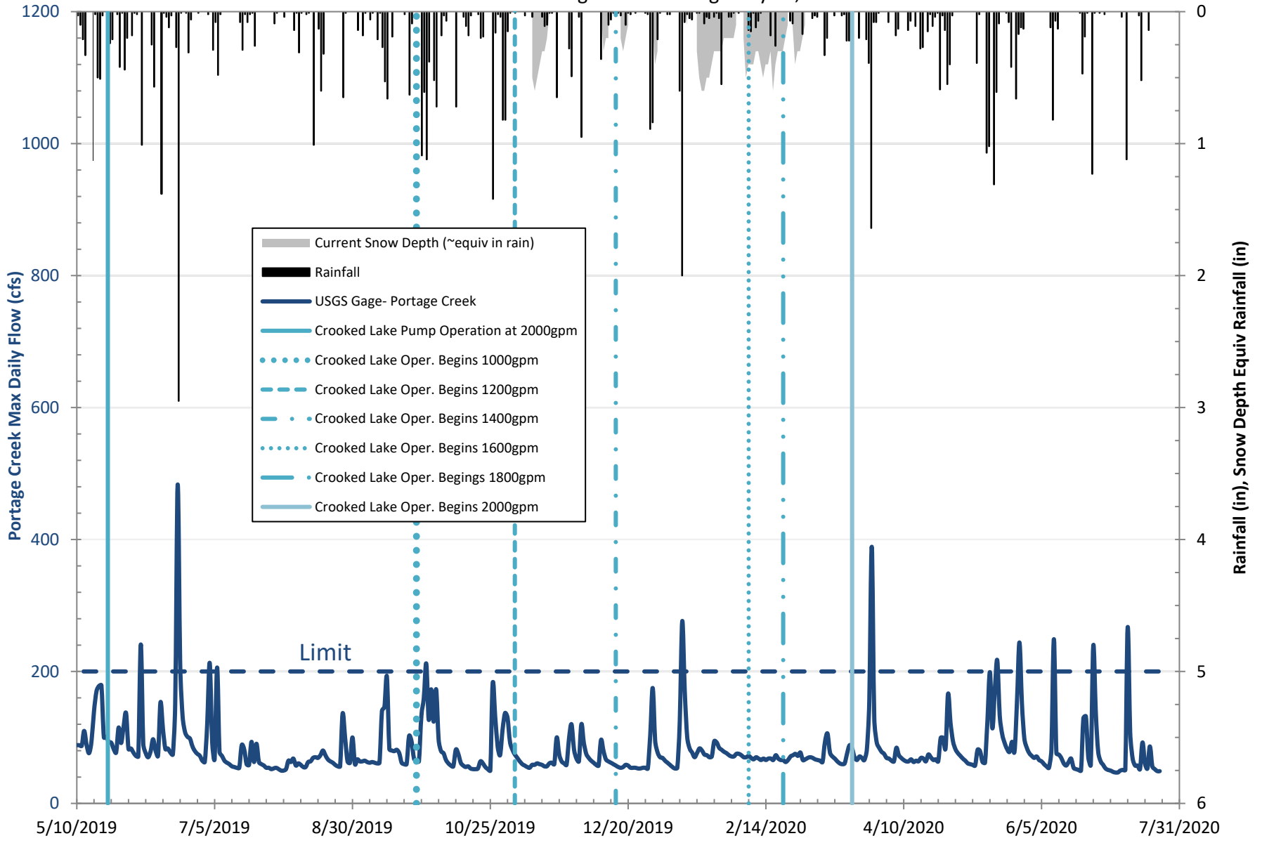
Charter Township of Texas Flood Study Figure USGS Monitoring Results through July 23, 2020
