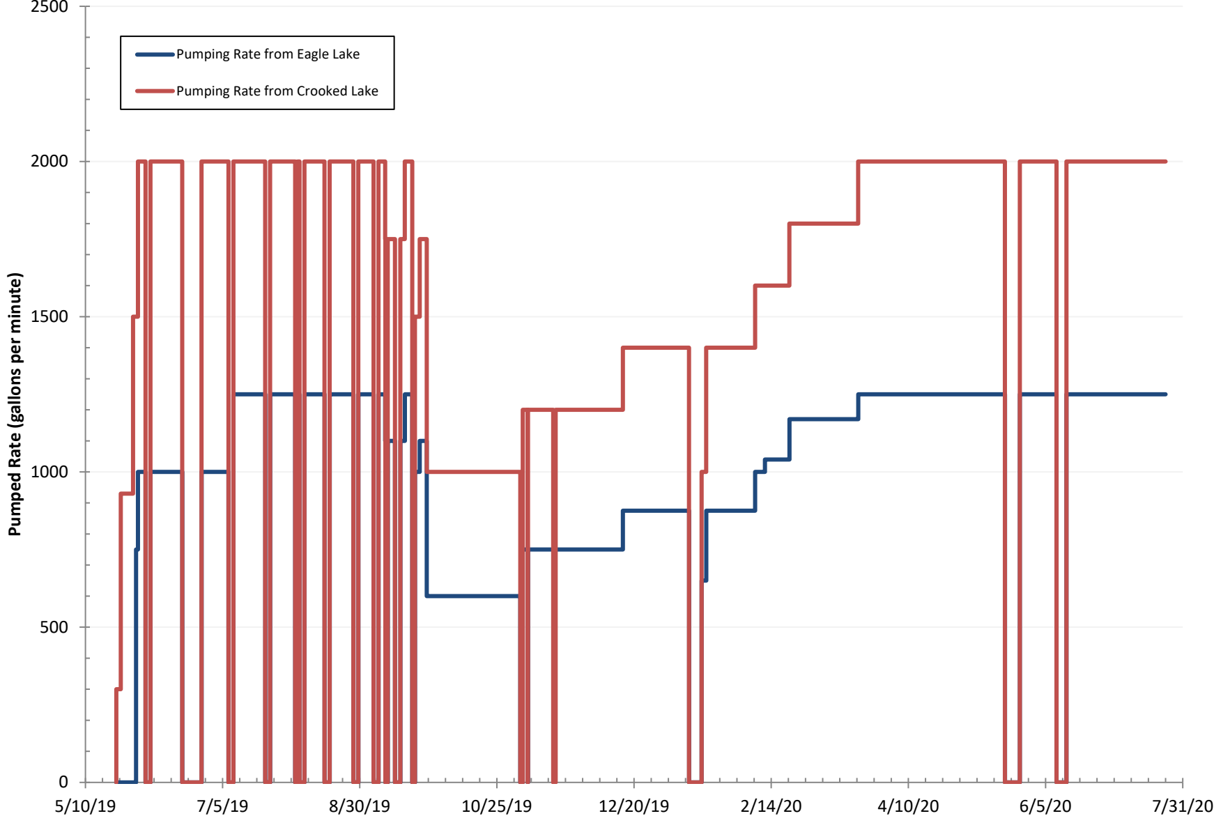
Charter Township of Texas Flood Study Figure Pumping Data through July 23, 2020
