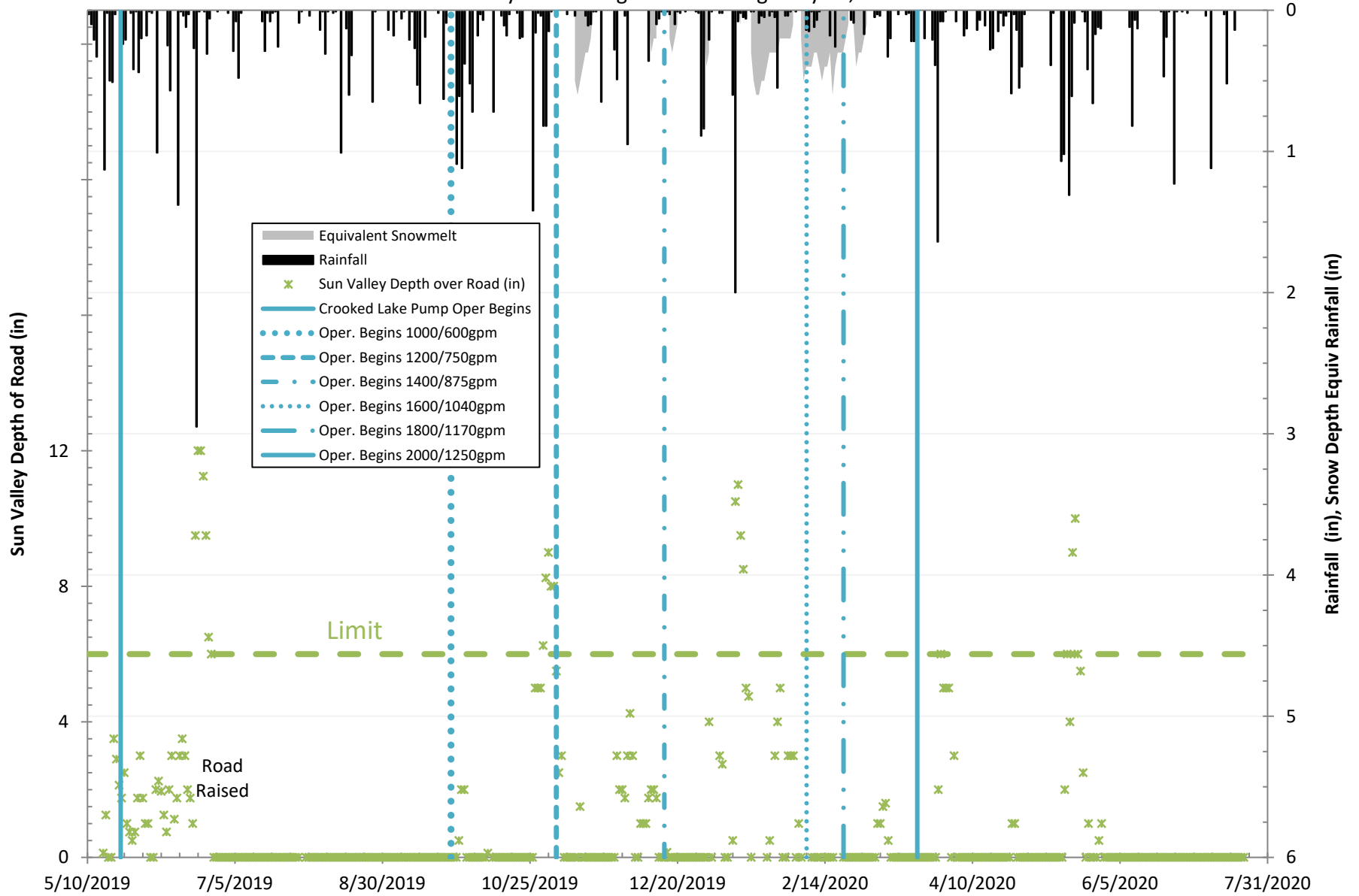
Charter Township of Texas Flood Study Figure Sun Valley Monitoring Results through July 23, 2020
