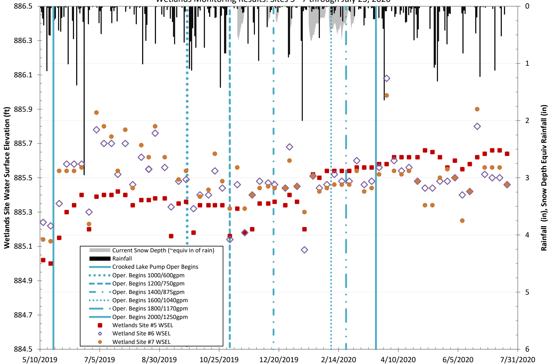
Wetlands Monitoring Results: Sites 5 - 7 through July 23, 2020
