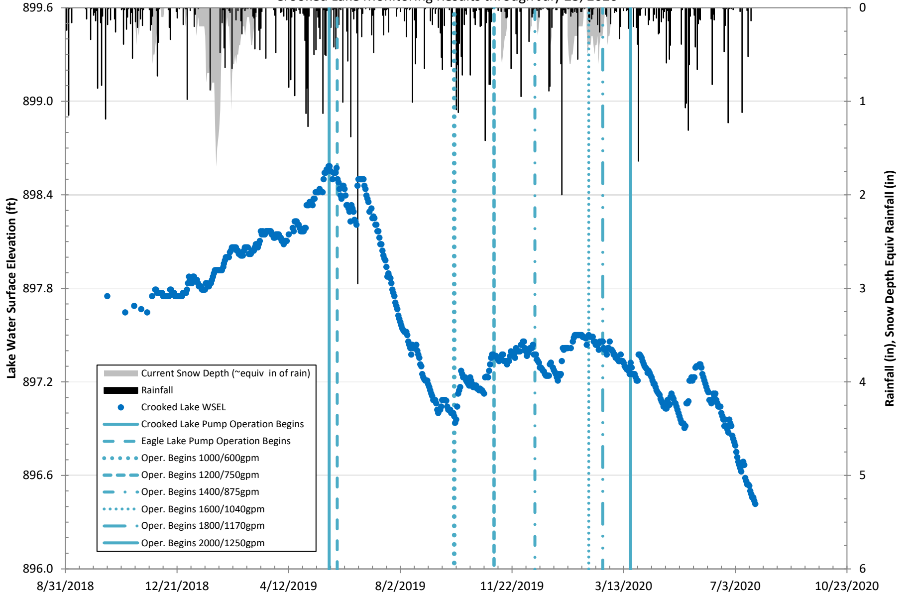
Charter Township of Texas Flood Study Figure Crooked Lake Monitoring Results through July 23, 2020
