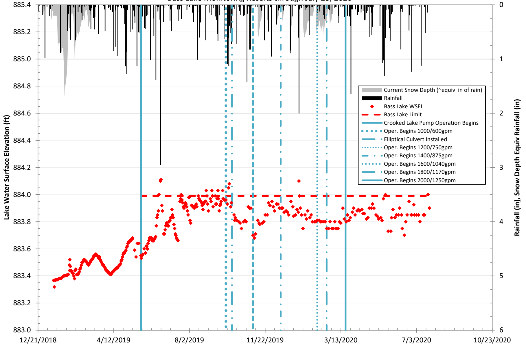
Charter Township of Texas Flood Study Figure Bass Lake Monitoring Results through July 23, 2020
